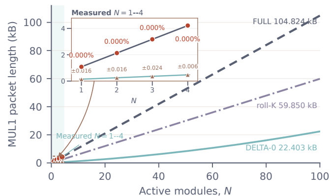
(a) Packet length
