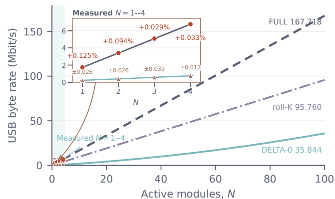
(b) USB application rate at 200 Hz
