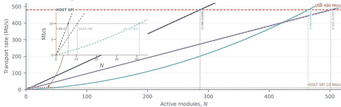
(c) Total transport rate at 200 Hz
